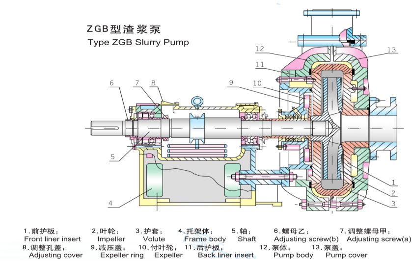
Horizontal Double Casing Slurry Pumps Structure of ZGB Series
