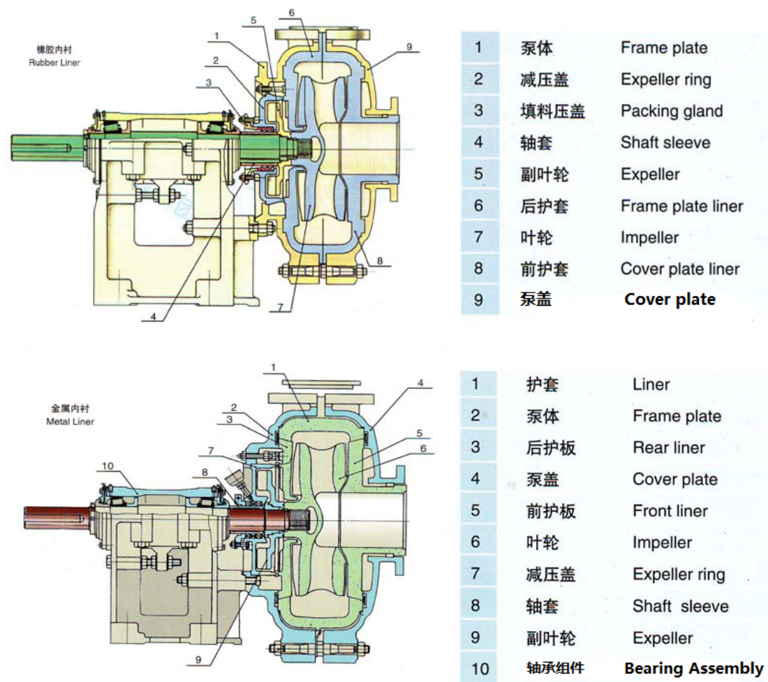
Horizontal Double Casing Slurry Pumps Structure of ZGB Series
